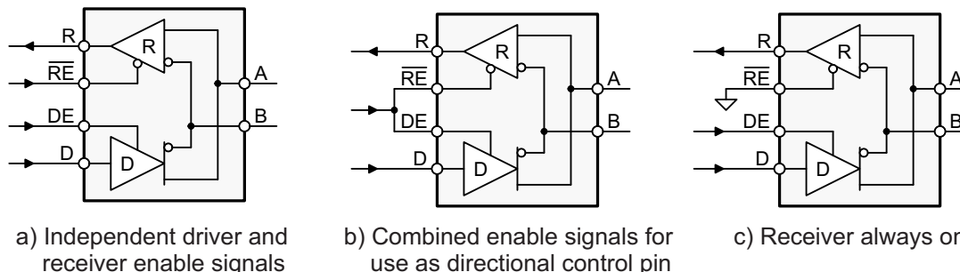
Figure 18. Transceiver Configurations
