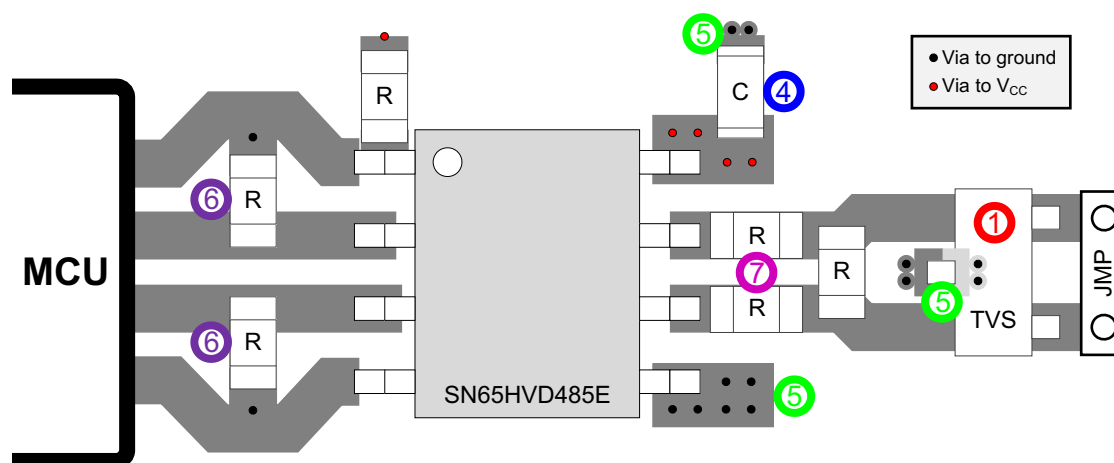
Figure 22. Layout Example
