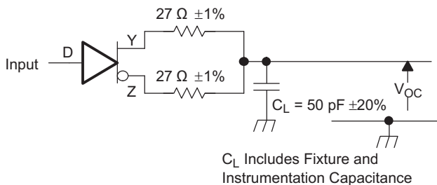
Figure 4. Test Circuit and Definitions for the Driver Common-Mode Output Voltage
