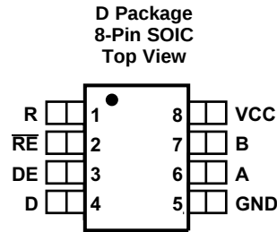
Pin Functions
