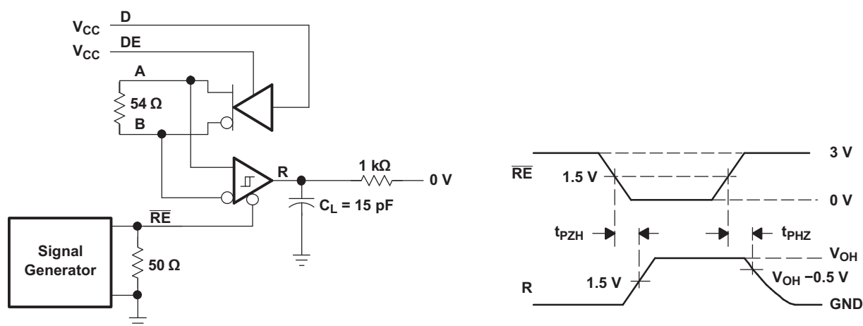
Figure 18. Receiver Enable Test Circuit and Waveforms, Data Output High (Driver Active)
