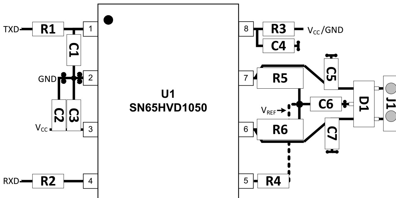
Figure 31. Layout Example
