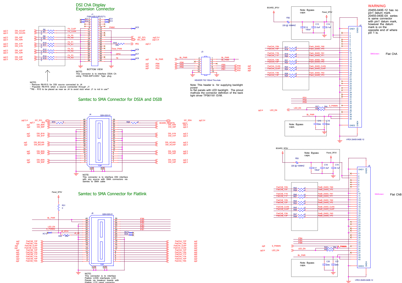
Figure 5. SN65DSI8X Schematic 2
