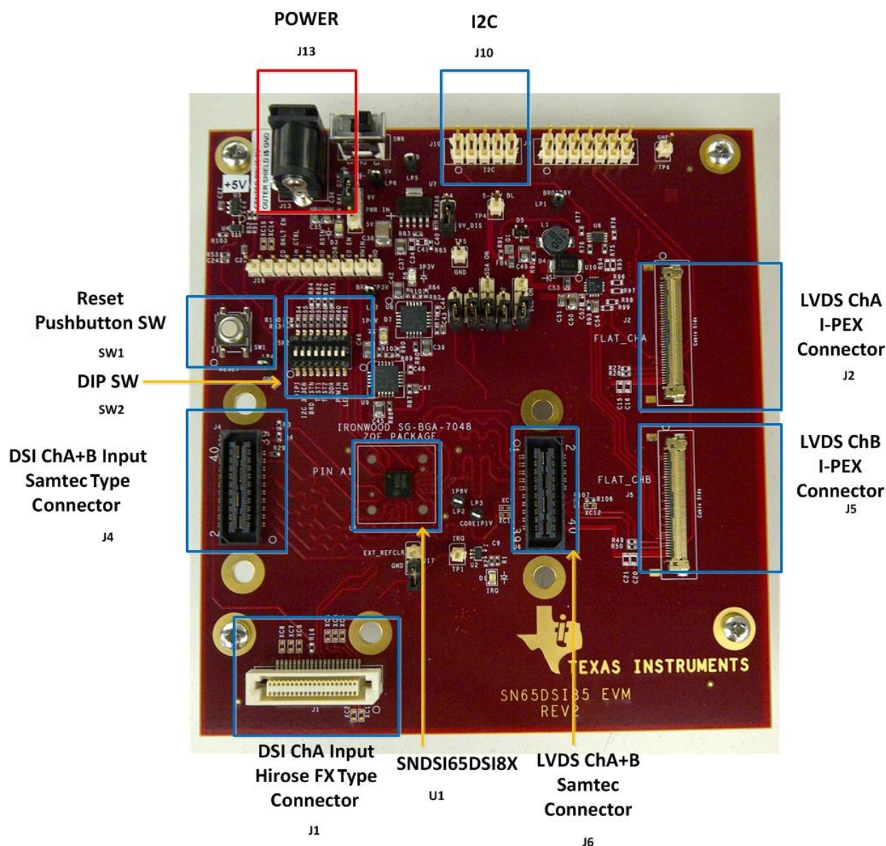
Figure 1. SN65DSI8XEVM
