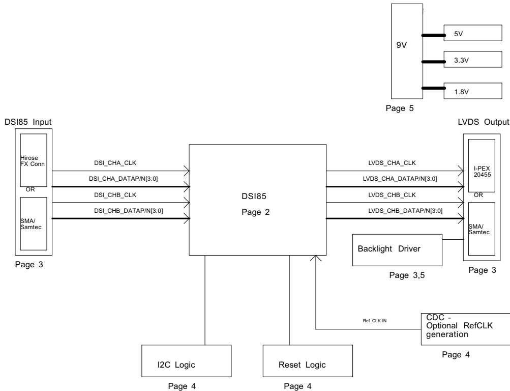
Figure 2. SN65DSI8X EVM Block Diagram
