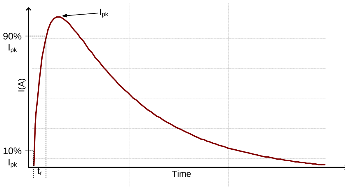
Figure 6. HBM Curve
