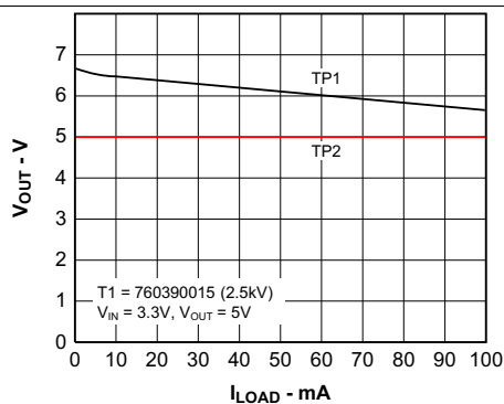
Figure 9. Output Voltage vs Load Current
