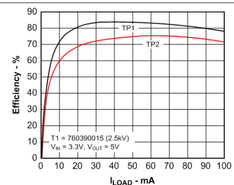
Figure 10. Efficiency vs Load Current
