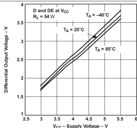
Figure 2. Differential Output Voltage vs Supply Voltage
