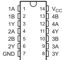
D, DB, NS, J, W, or PW Package 14-Pin SOIC, SSOP, SOP, CDIP, or TSSOP Top View
