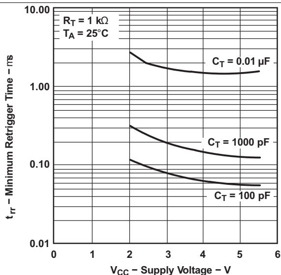
Figure 1. Minimum Trigger vs V_{CC} Characteristics
