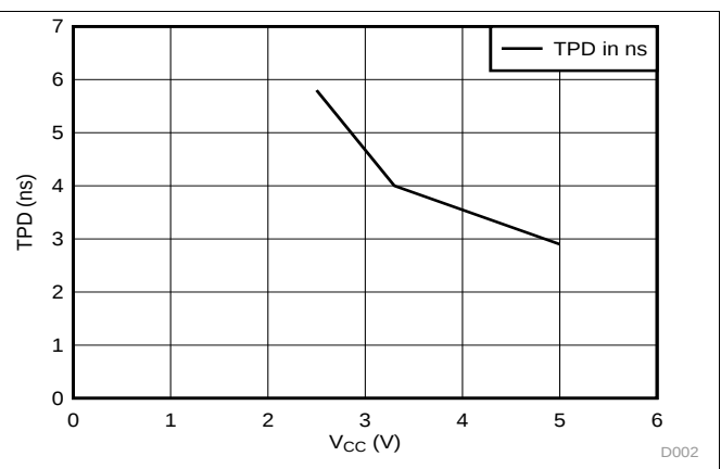
Figure 2. TPD vs V_{CC} at 25^\circ\text{C}
