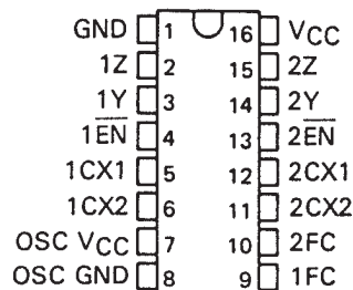
SN54LS626 . . . J OR W PACKAGE SN74LS626 . . . D OR N PACKAGE
