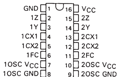
SN54LS626 . . . J OR W PACKAGE SN74LS626 . . . D OR N PACKAGE
