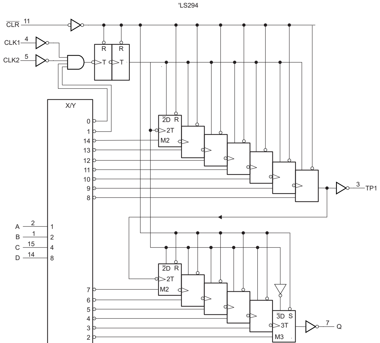
Figure 6. Logic Diagram (Positive Logic) SN74LS294
