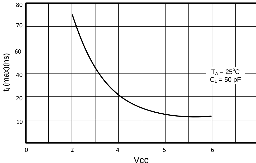
Figure 1. t_t vs V_{CC}
