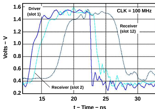
Figure 5. Source-Synchronous Clock
