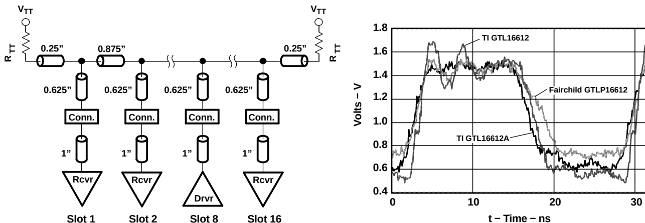
Figure 1. Test Backplane Model With Output Waveform Results
