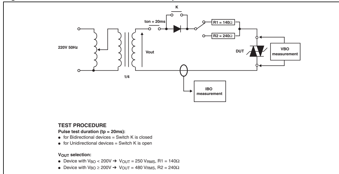
Figure 10. Test circuit 2 for IBO and VBO parameters
