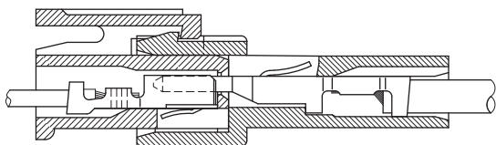
TERMINAL ASSEMBLY DRAWING
