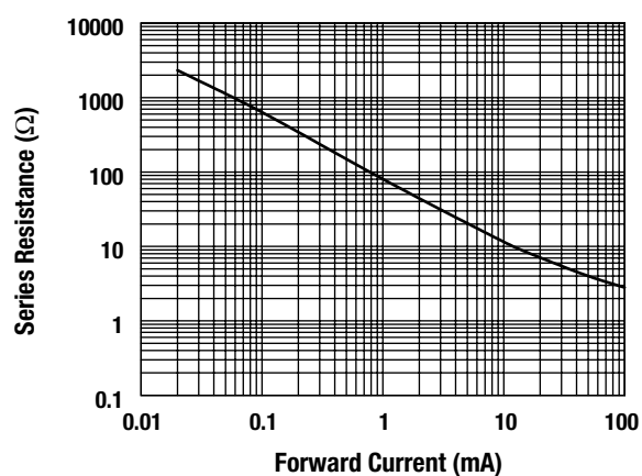
Series Resistance vs. Current @ 100 MHz
