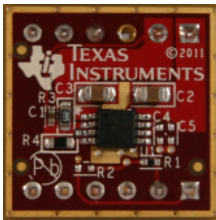
Figure 1. SMP-TPS7A4001-MVK Submodule
