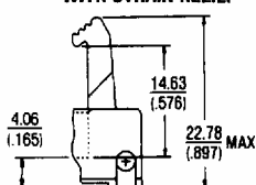
STYLE 2 WITH STRAIN RELIEF
