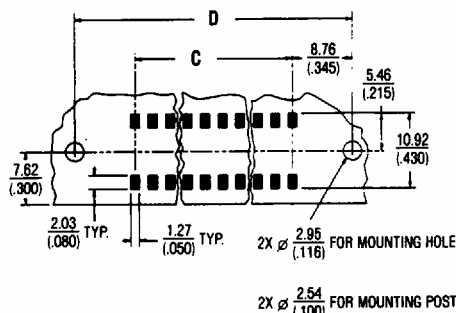
RECOMMENDED PAD PATTERN
