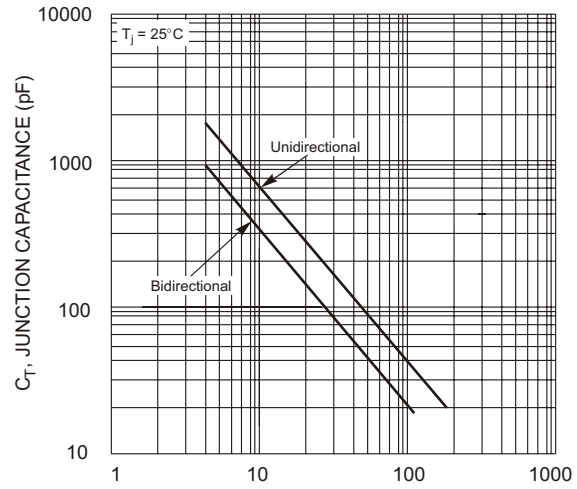
Fig. 2 Typical Total Capacitance
