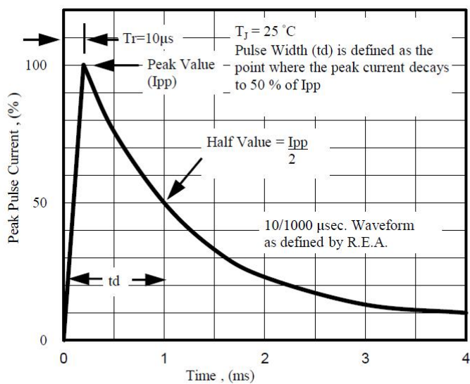
Fig. 5 - Pulse Waveform
