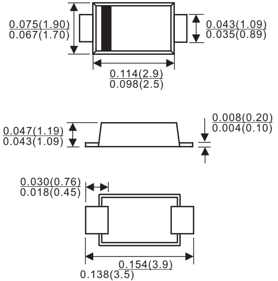
SOD-123FL
