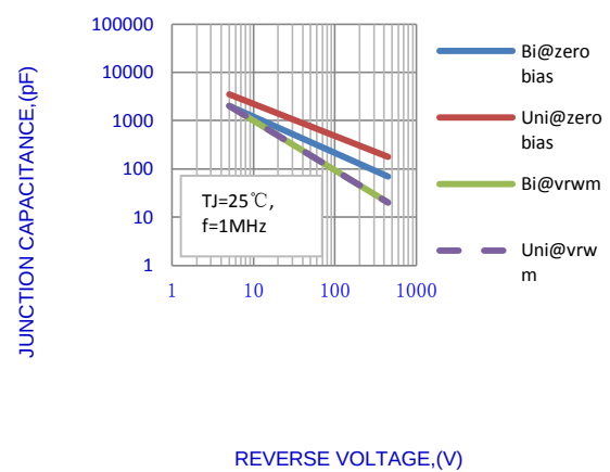
Fig.6-TYPICAL JUNCTION CAPACITANCE
