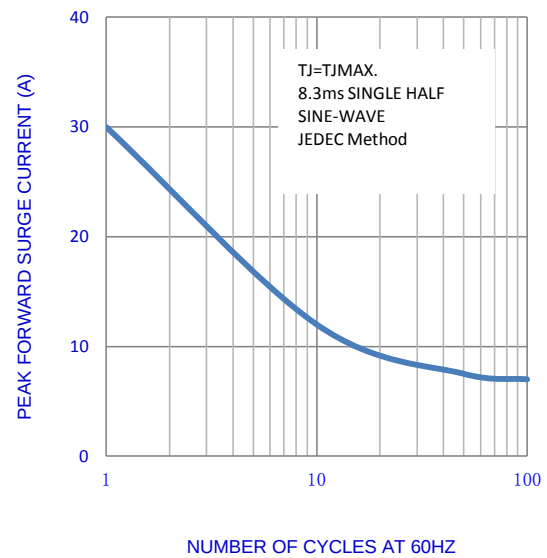
Fig.4-MAX. NON-REPETITIVE SURGE CURRENT
