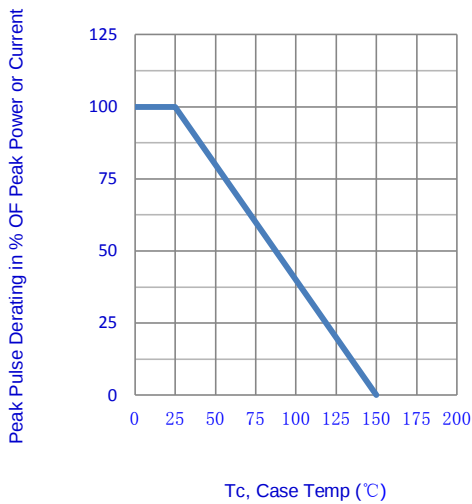
Fig.1-Pulse Derating Curve
