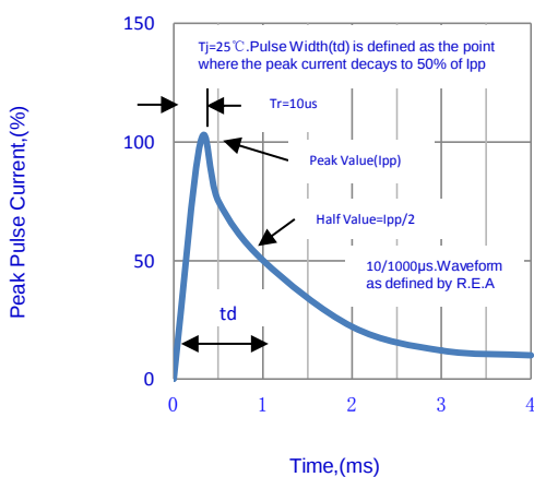
Fig.5-Pulse Waveform
