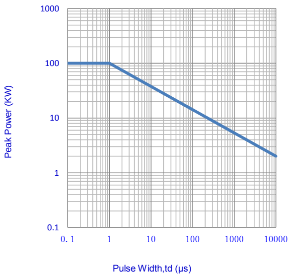
Fig.3- Peak Pulse Power Rating Curve
