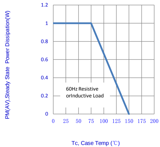
Fig.2- Steady State Power Derating Curve
