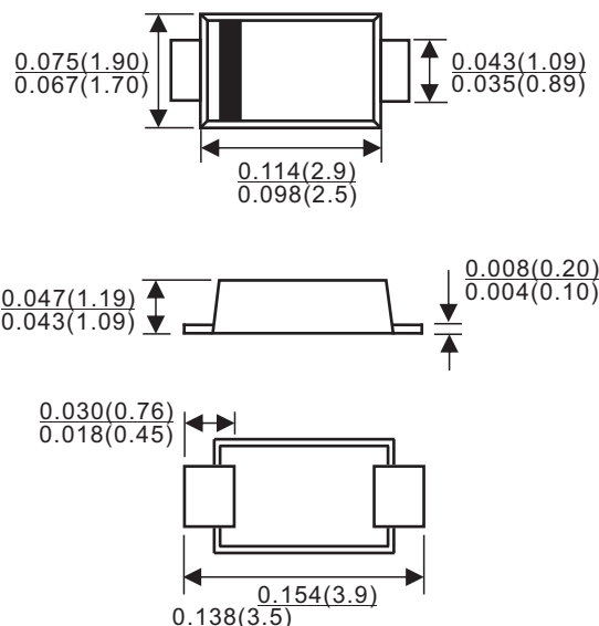
SOD-123FL
