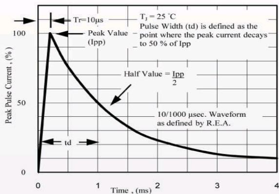
Fig. 5 - Pulse Waveform
