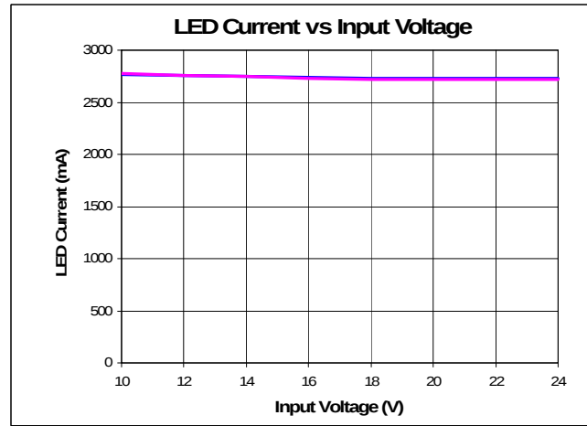
Figure 41: Line regulation
