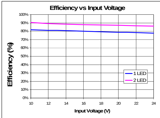
Figure 40: Efficiency
