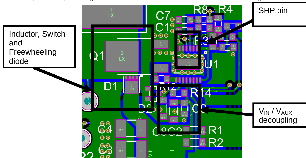
Figure 38: Circuit Layout
