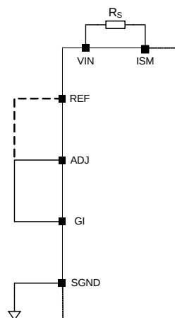
Figure 17: Buck configuration
