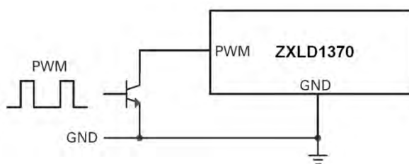
Figure 29: PWM dimming from open collector switch
