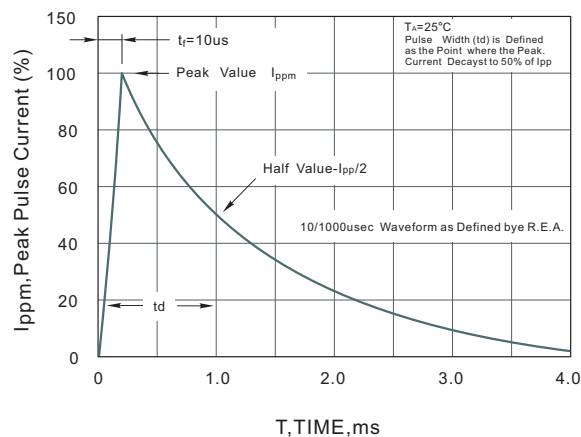
Fig.2 Pulse Waveform
