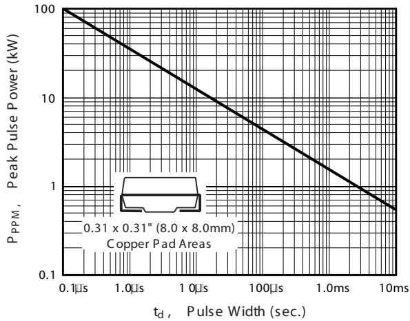
Fig. 1D Peak Pulse Power Rating Curve
