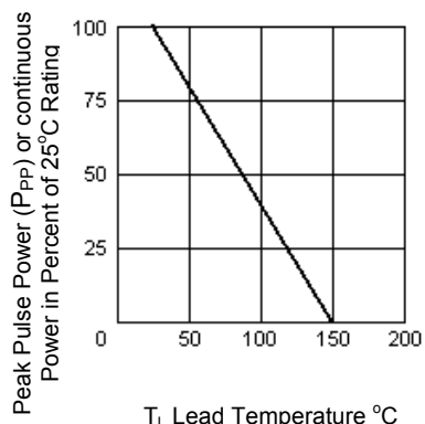
FIGURE 3 - Derating Curve
