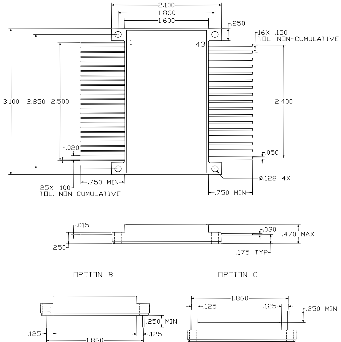
Fig. 3: Mechanical Outline For Plastic Case Package, SMC6MXX-XX-1
