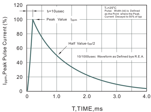
Fig.3 Pulse Waveform
