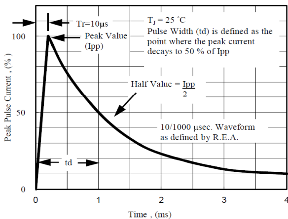
Fig. 5 - Pulse Waveform
