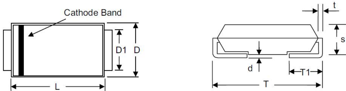
SMB/DO-214AA
