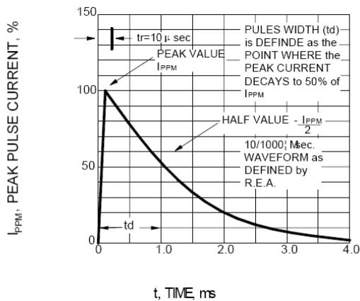
FIG.3 -- PULSE WAVEFORM
