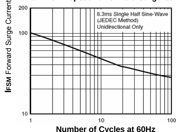
4- Max. Non-Repetitive Forward Surge Current
