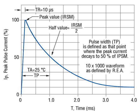
Figure 4- Pulse Waveform
