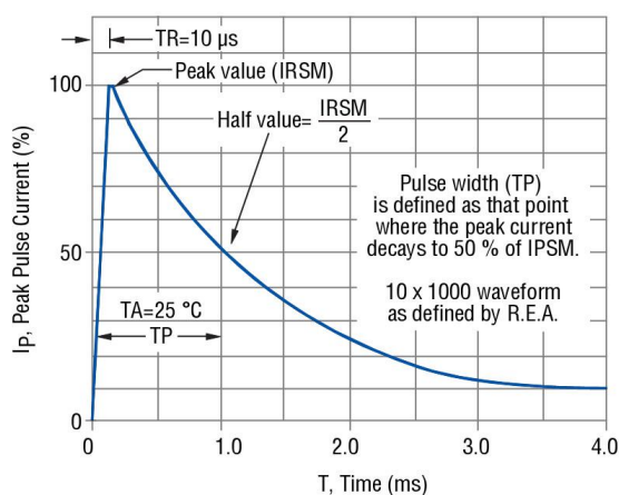
Figure 4- Pulse Waveform
