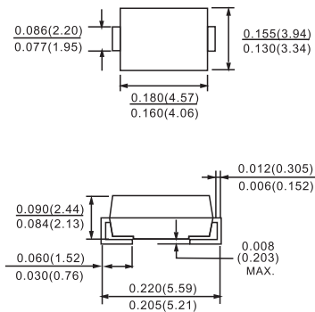
DO-214AA(SMB)
