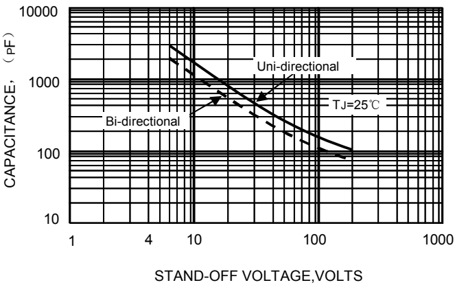
FIG.4-TYPICAL JUNCTION CAPACITANCE
