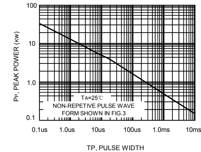
FIG.5-PULSE RATING CURVE
