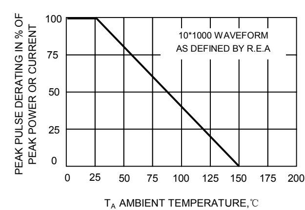
FIG.1-PULSE DERATING CURVE
