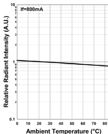
Rel. Radiant Intensity vs. Ambient Temperature
