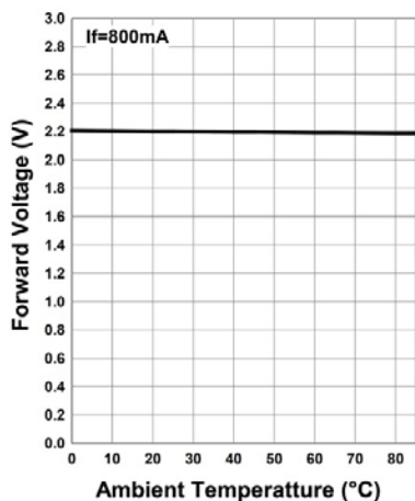
Forward Voltage vs. Ambient Temperature
