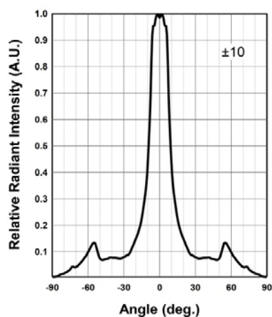
Radiation Characteristics
