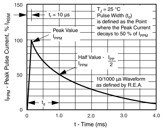
Figure 3. Pulse Waveform
