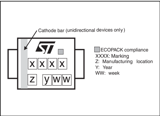
Figure 18. Marking layout (1)
