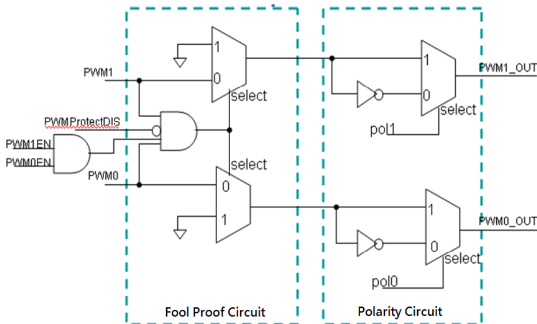
Fig. 13-2: Opertion of the PWM Protect Mode
