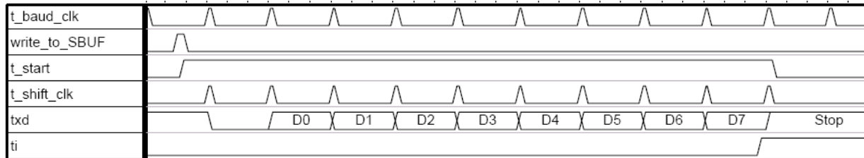
Fig. 9-3: Transmit mode 1
