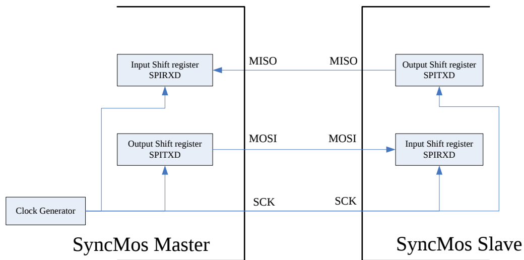
Fig. 15-2: SPI Mater and slave transfer method
