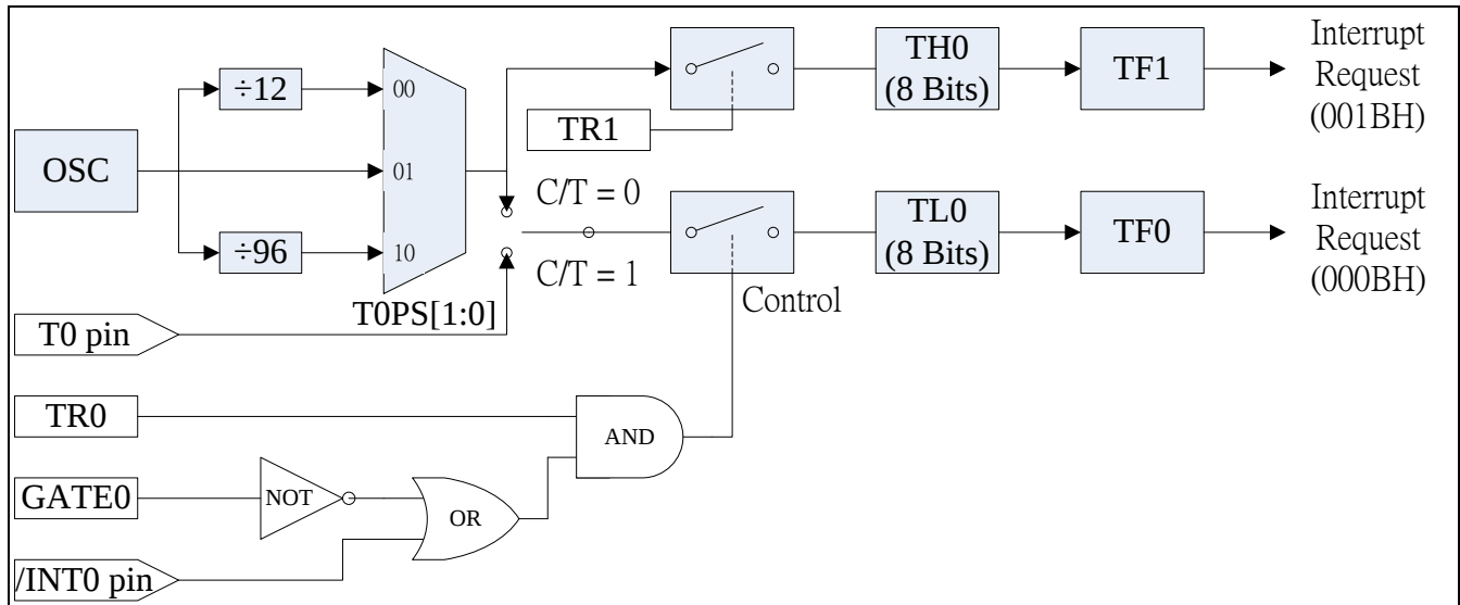
Fig. 7-4: Mode 3 Timer 0 acts as two independent 8 bit Timers / Counters operating
