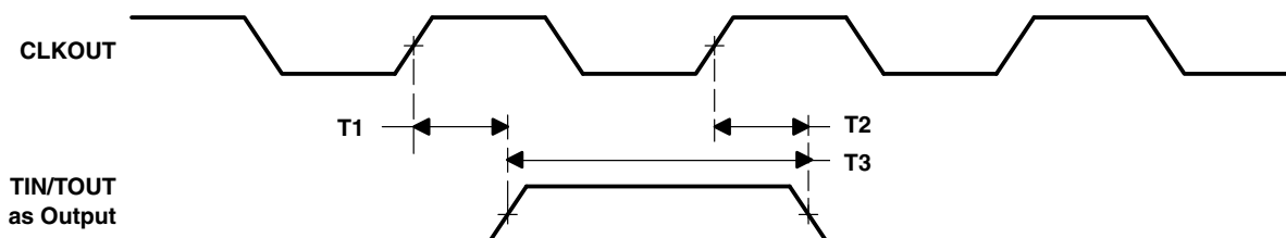
Figure 5–18. TIN/TOUT Timing When Configured as Outputs
