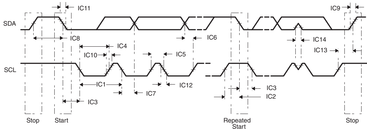
Figure 5-37. I²C Receive Timings
