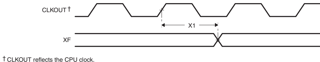
Figure 5-20. XF Timings
