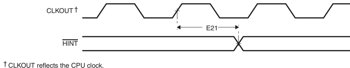
Figure 5-31. \overline{\text{HINT}} Timings
