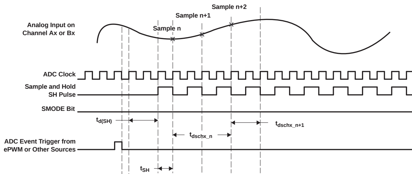
Figure 6-24. Sequential Sampling Mode (Single-Channel) Timing
