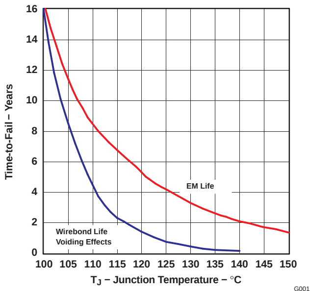
Figure 6-1. Wirebond / EM Life for SM320F280xPZMEP
