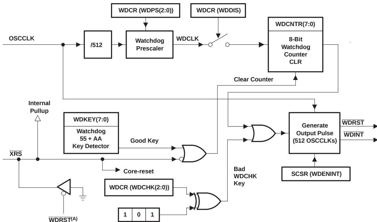
Figure 3-12. Watchdog Module
