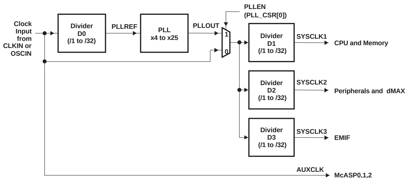
Figure 4-45. PLL Topology
