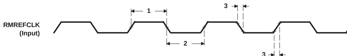
Figure 7-65. RMREFCLK Timing
